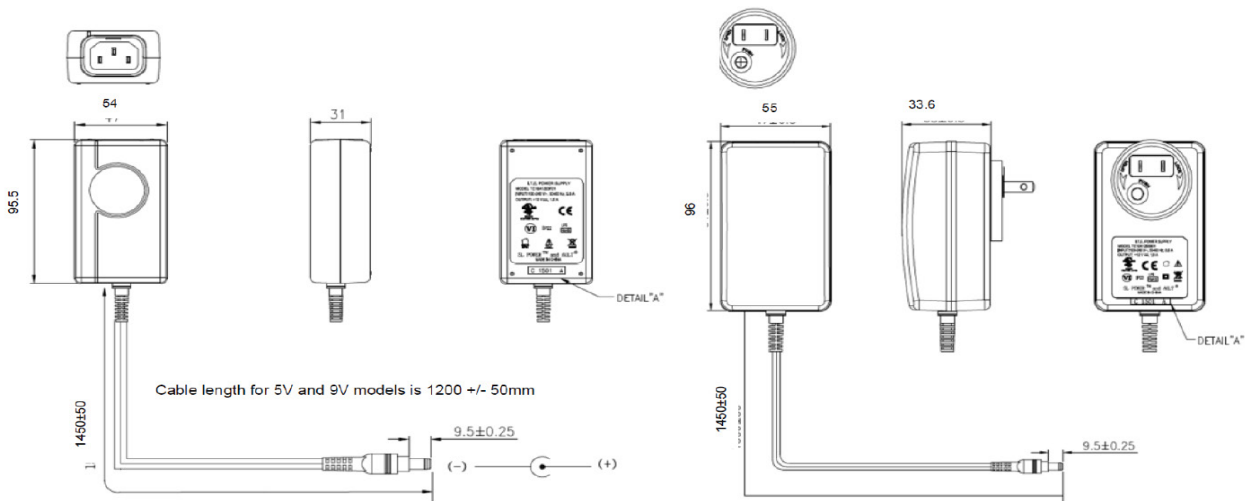
IEC60320 C14 Receptacle, 2.5mm x 5.5mm x 9.5mm Barrel Connector Interchangeable N.A. Blade, 2.5mm x 5.5mm x 9.5mm Barrel Connector
