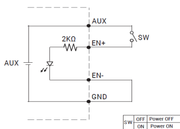
(A) Using internal 5V auxiliary source
