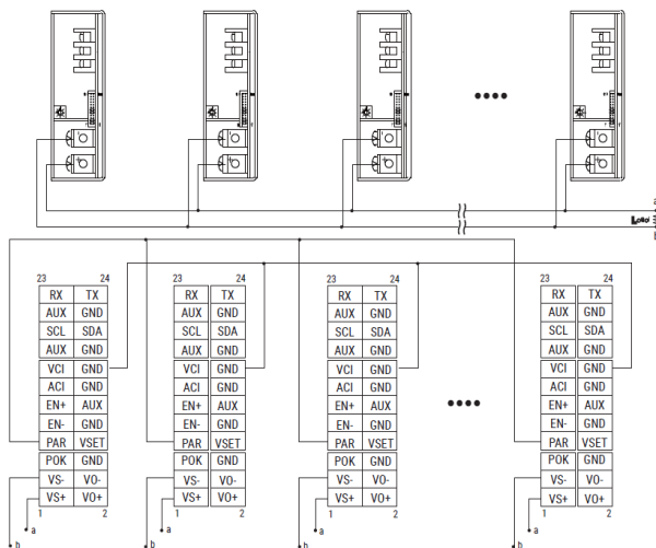
Current Sharing with Remote Sensing (Parallel Connection)
