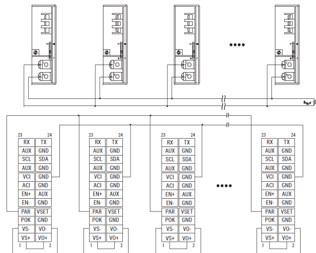
Current Sharing with Local Sensing
