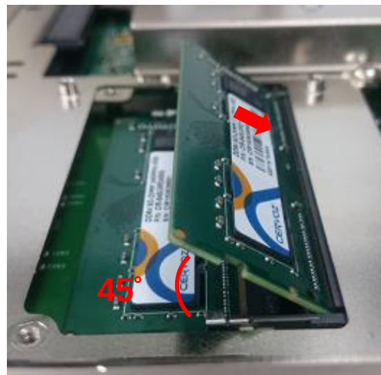
Upper socket
