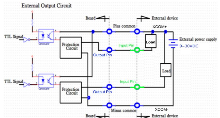
Digital Output Wiring
